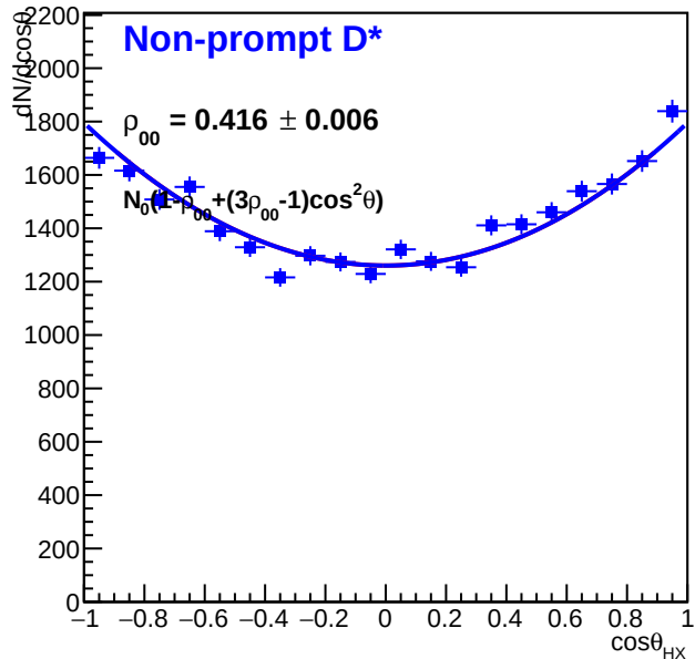
Non-prompt D* ( 7 < p_T < 10 GeV/c)
