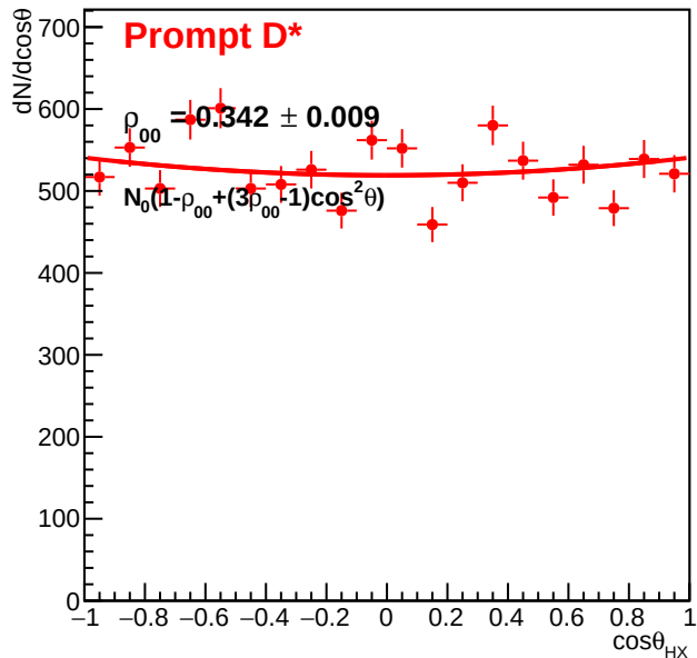
Prompt D* ( 7 < p_T < 10 GeV/c)
