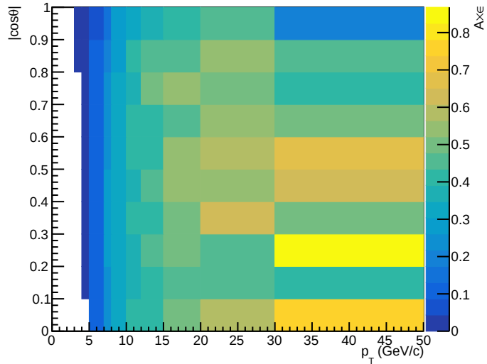
prompt D^*
