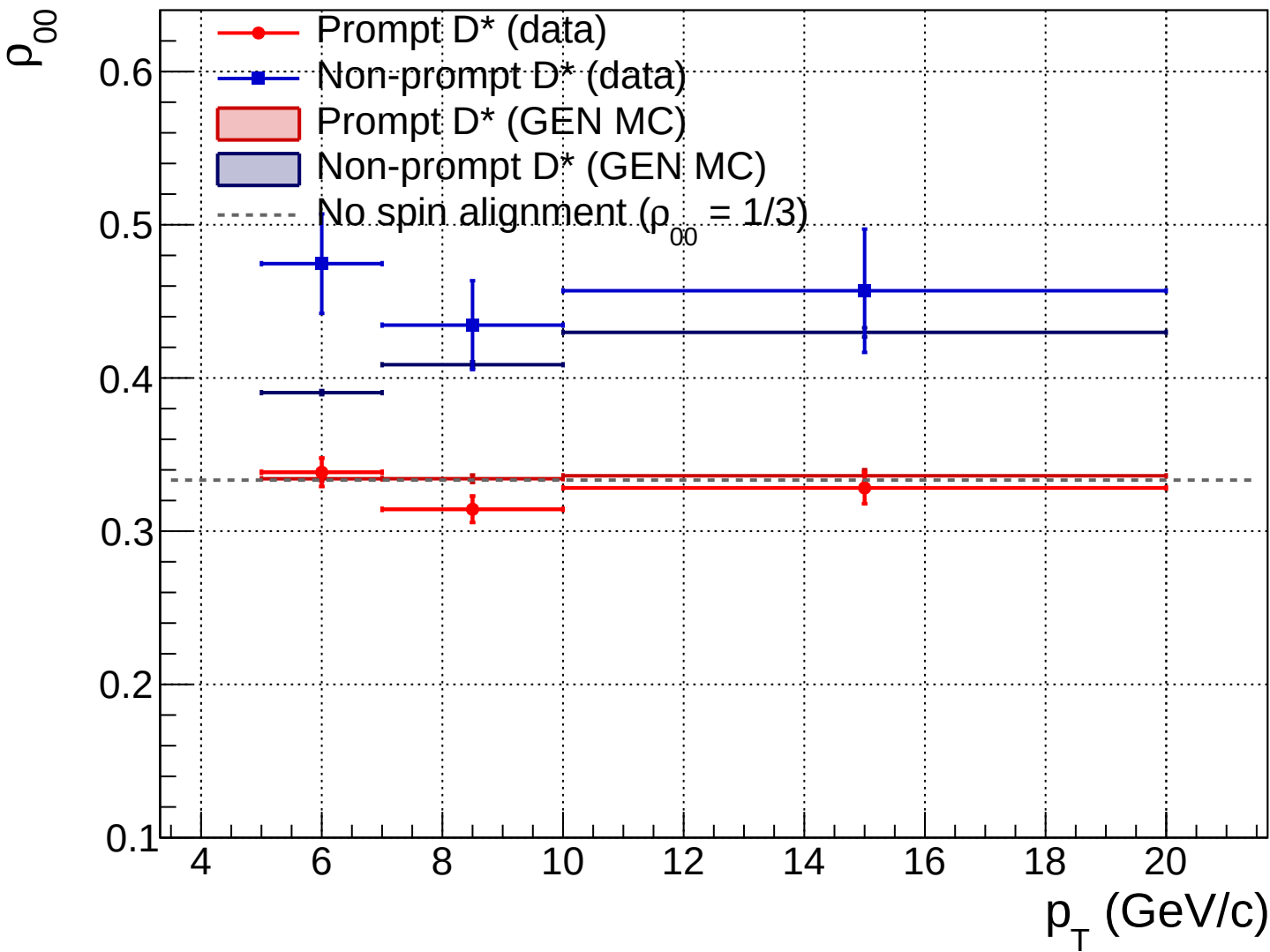
\rho_{00} vs p_T
