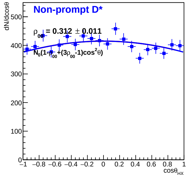
Non-prompt D* ( 10 < p_T < 20 GeV/c)
