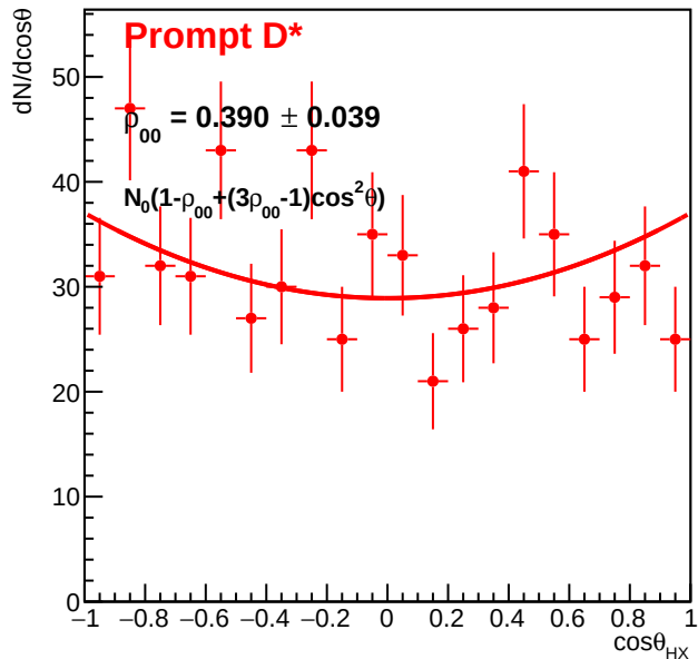
Prompt D* ( 10 < p_T < 20 GeV/c)
