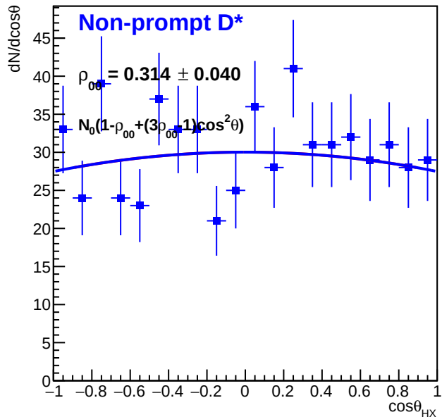
Non-prompt D* ( 20 < p_T < 50 GeV/c)
