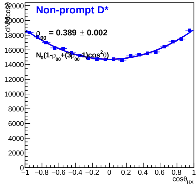
Non-prompt D* ( 5 < p_T < 7 GeV/c)
