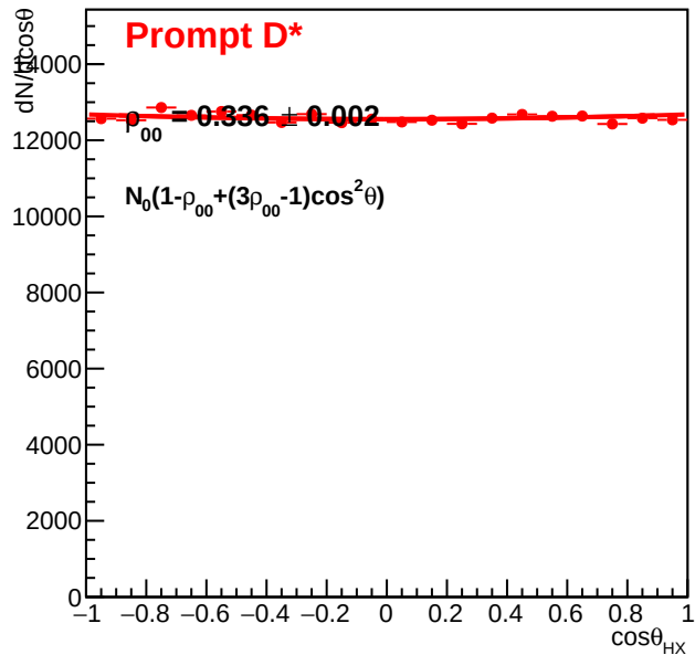
Prompt D* ( 5 < p_T < 7 GeV/c)
