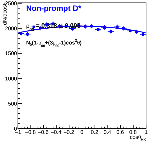
Non-prompt D* ( 5 < p_T < 7 GeV/c)
