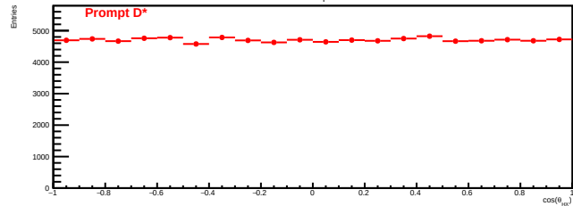
Prompt D* ( 10 < p_T < 20 GeV/c)
