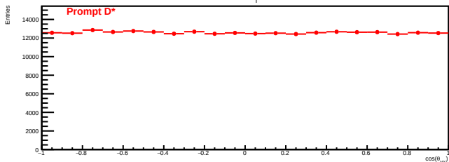
Prompt D* ( 7 < p_T < 10 GeV/c)
