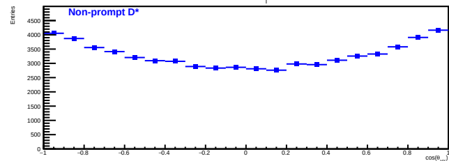
Non-prompt D* ( 20 < p_T < 50 GeV/c)
