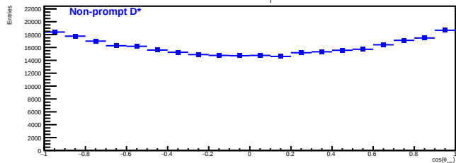
Non-prompt D* ( 7 < p_T < 10 GeV/c)
