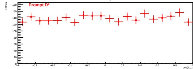
Prompt D* ( 20 < p_T < 50 GeV/c)
