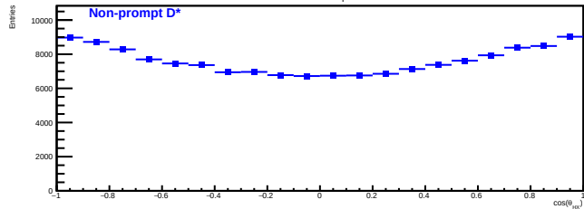
Non-prompt D* ( 10 < p_T < 20 GeV/c)
