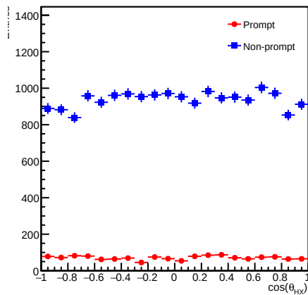
7 < p_T < 10 \text{ GeV/c}
