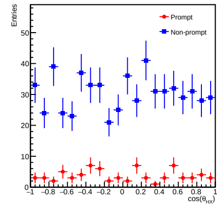
20 < p_T < 50 \text{ GeV/c}
