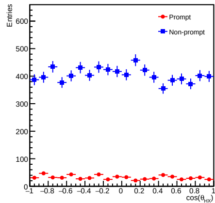
10 < p_T < 20 \text{ GeV/c}
