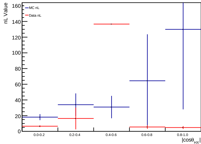
nL for 5.000000 < p_T < 7.000000
