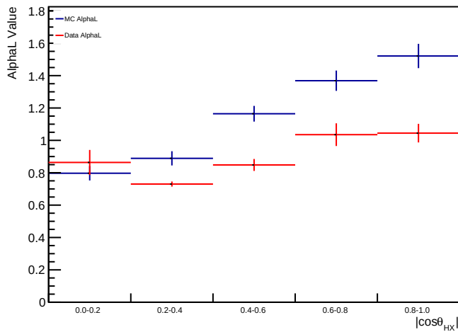
AlphaL for 7.000000 < pT < 10.000000
