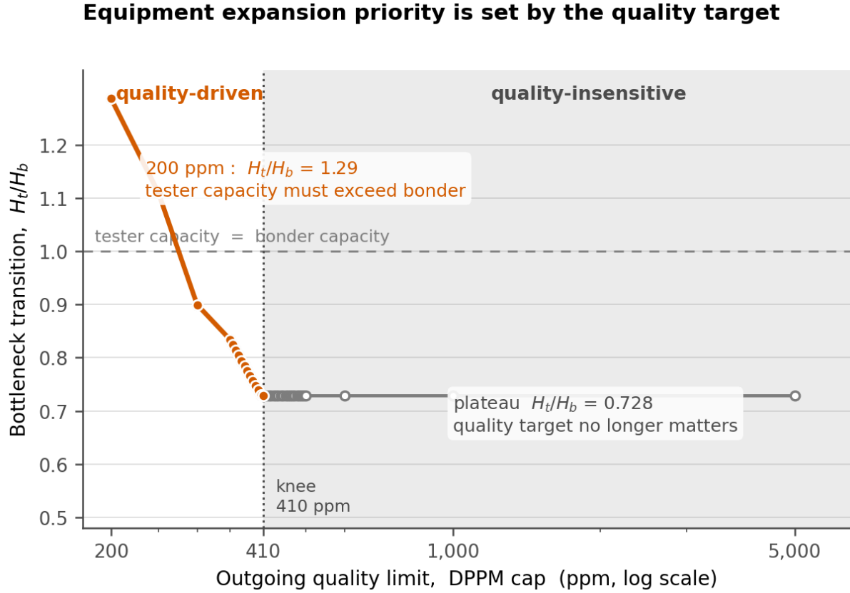
Fig. 1. Bottleneck transition ratio versus outgoing quality limit. Below the transition ratio the tester is the bottleneck; above it the bonder is. The curve is flat above the 410 ppm knee and rises steeply below it.
