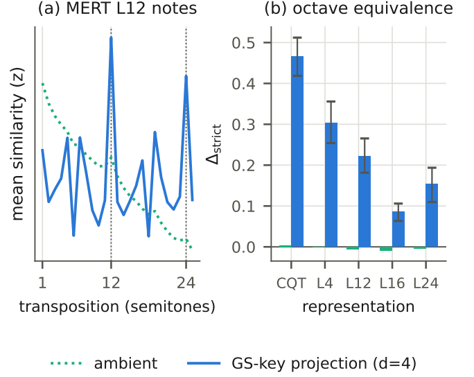
Fig. 2. Two views of the same rank-4 projection, fitted only on GiantSteps track tonics and applied unchanged to individual NSynth recordings. (a) Ambient similarity decays smoothly with transposition distance, while the projected curve reaches maxima at exactly twelve and twenty-four semitones. (b) The strict octave contrast that curve summarises, per representation, with instrument-bootstrap 95% intervals.
