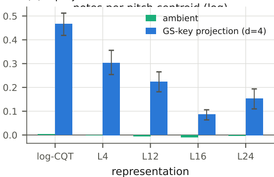
(b) a projection does
