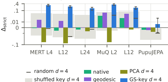
(b) octave equivalence, four metrics and two nulls
