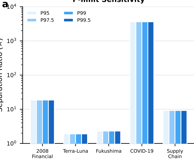
P-limit Sensitivity
