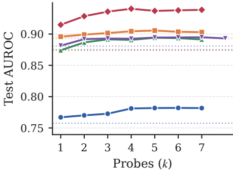
Qwen-2.5-7B
