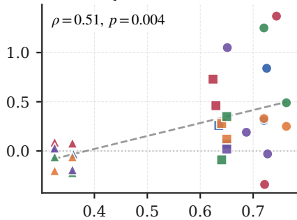
Qwen-2.5-7B
