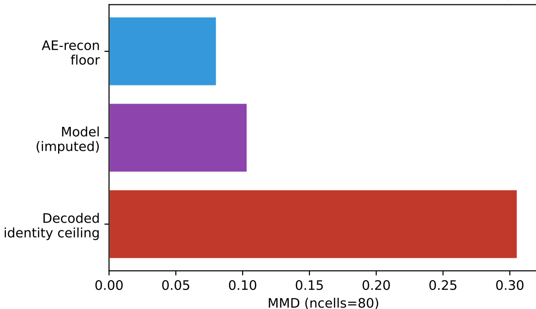
m1 v08 IMPACT — decoded-frame MMD ladder (model sits between AE floor and decoded ceiling)
