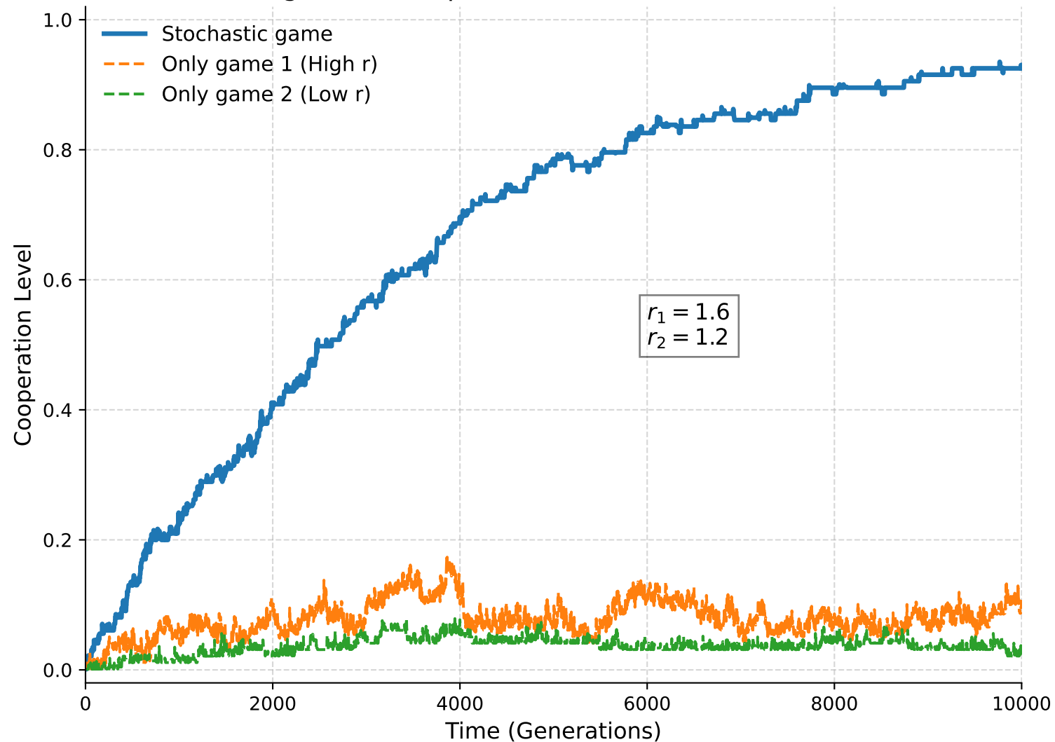
Figure 2: Group Game (Size=4, Beta=100.0)
