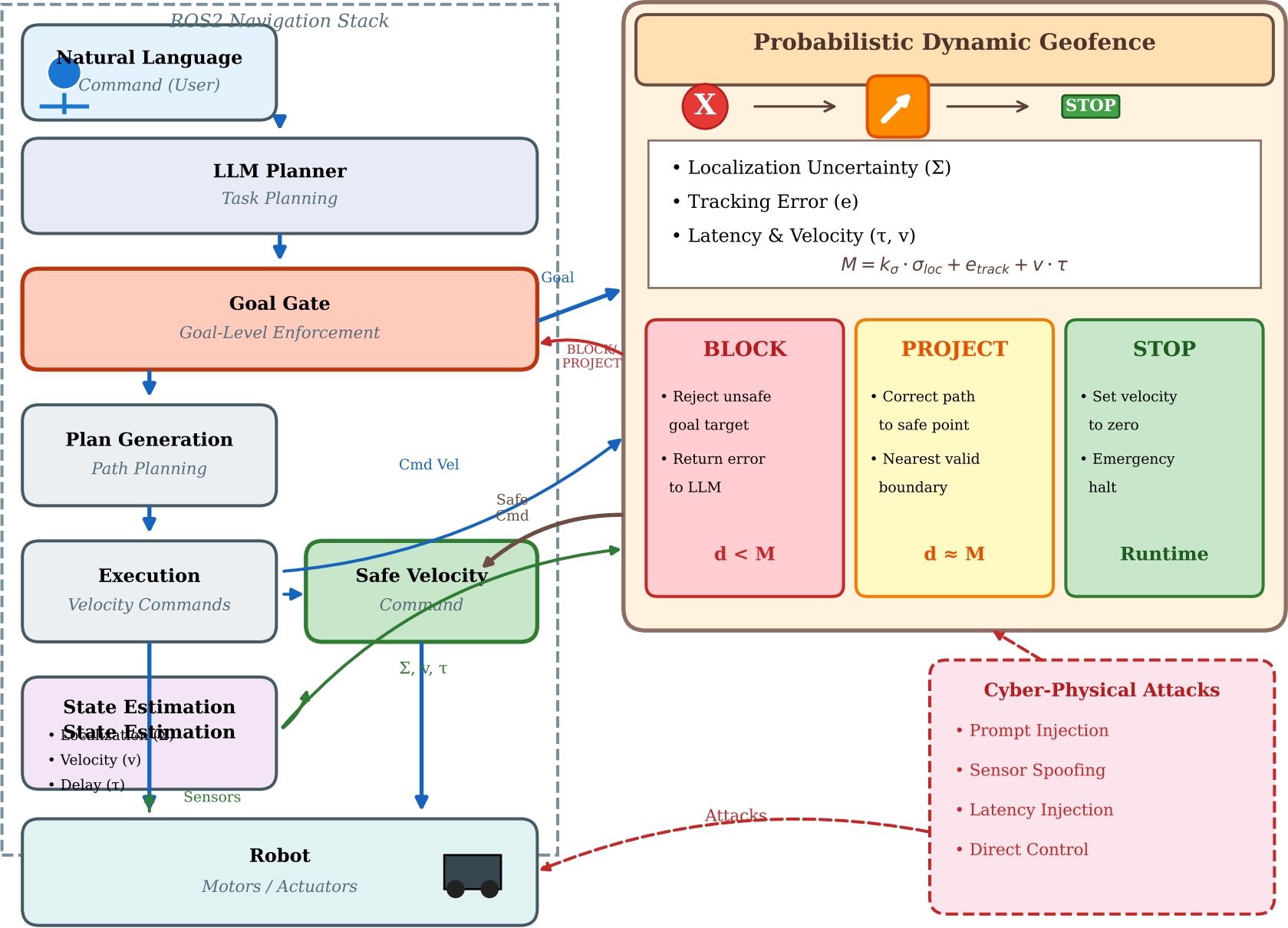
Figure X. Overview of LLM-based robot control system with probabilistic dynamic geofence. The geofence integrates with the standard pipeline (Plan Generation → Execution → Robot) to enforce spatial safety through BLOCK/PROJECT/STOP decisions.
