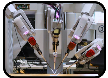
dVRK-Si
