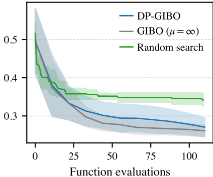
Validation loss
