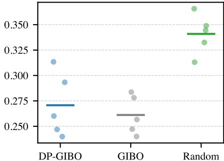
Final loss
