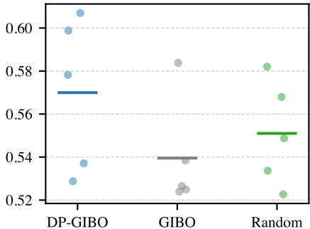
Final loss
