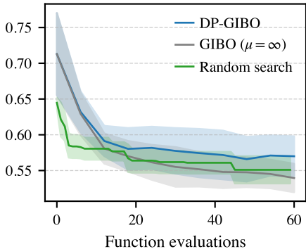
Validation loss
