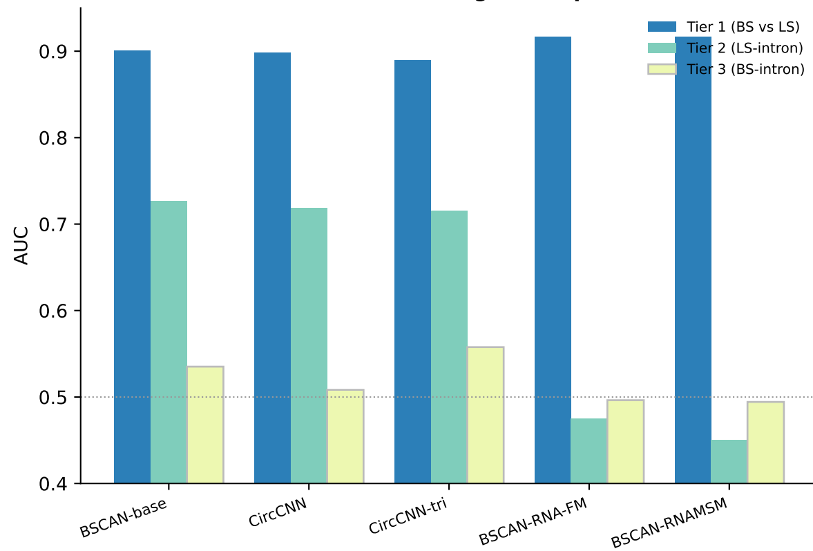
a Standard training: 3-tier probe
