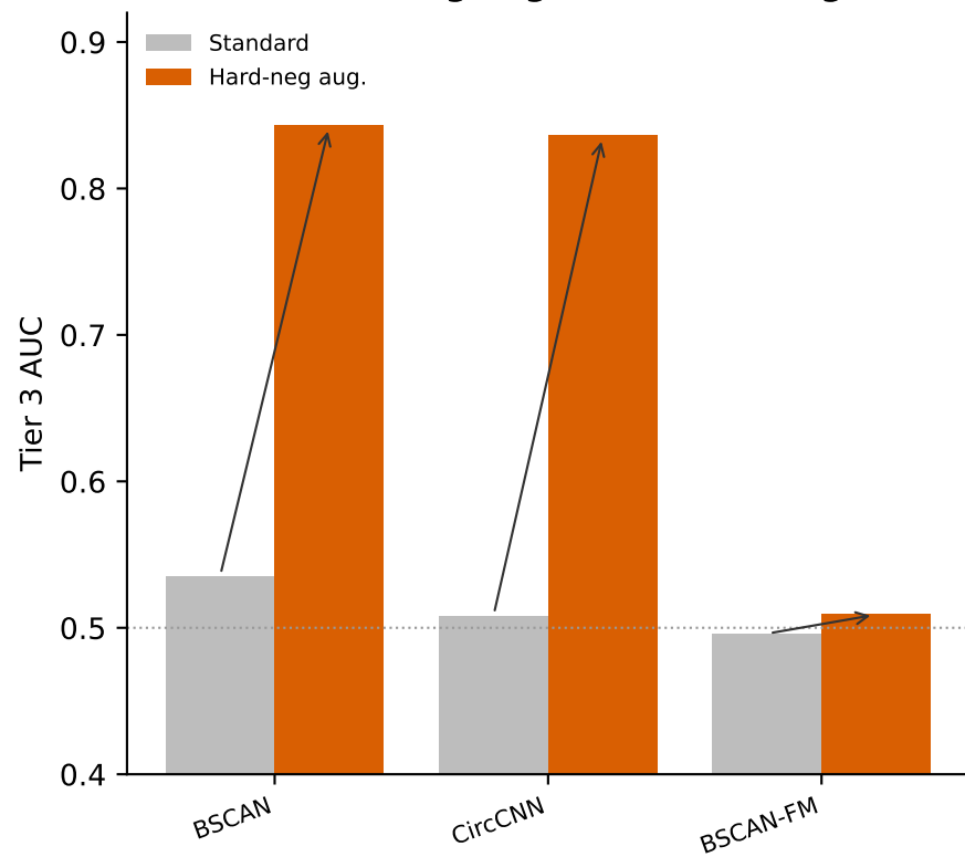
b Hard-neg augmented training
