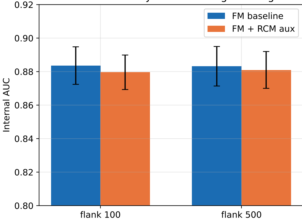
AUG-RCM: auxiliary RCM branch gives no gain
