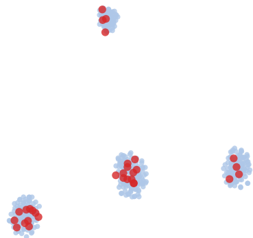
RNABERT (fine-tuned)
