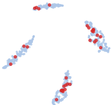
RNAErnie (fine-tuned)
