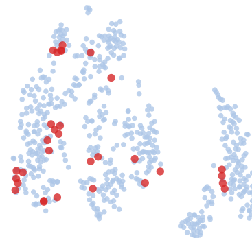
RNA-FM (fine-tuned)
