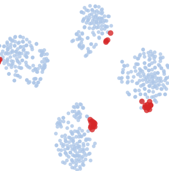
circMAC (ours)
