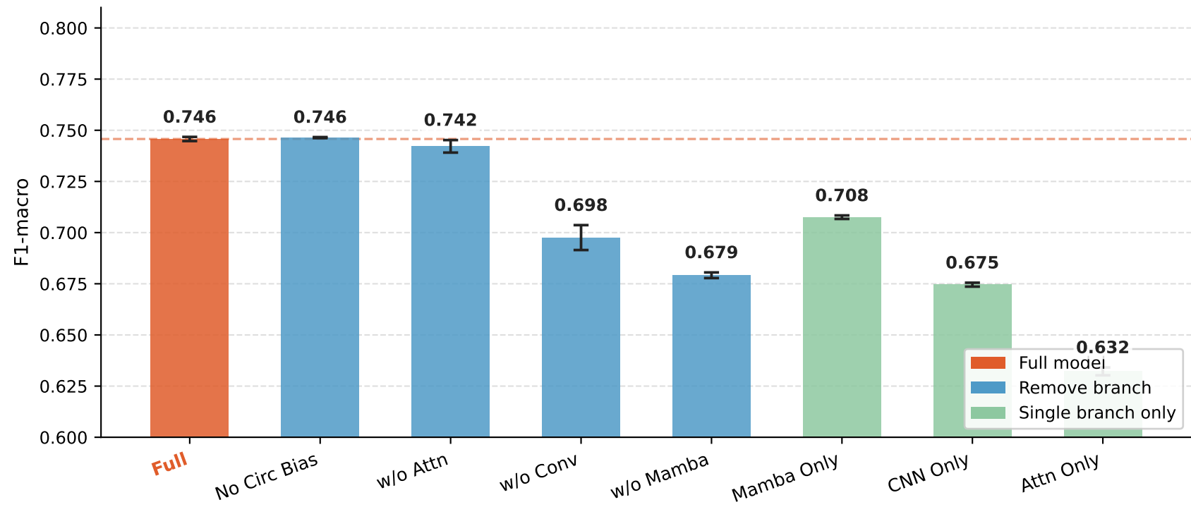
CircMAC Module Ablation
