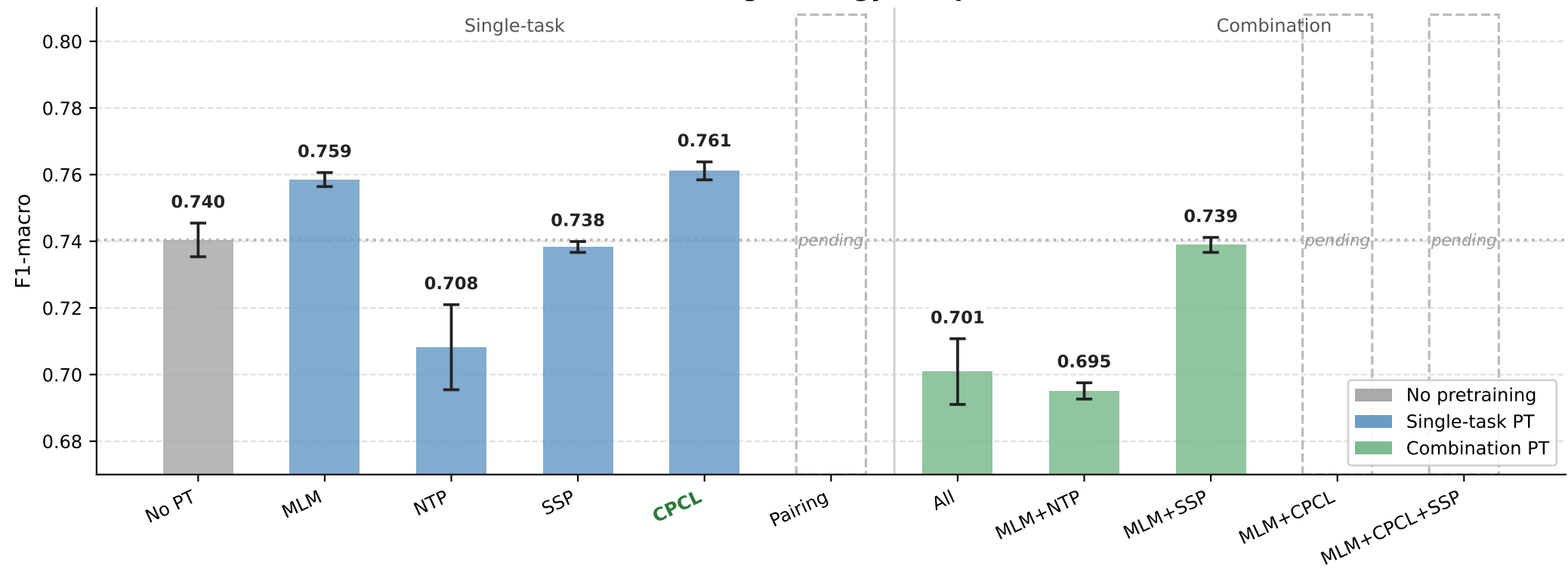
Pretraining Strategy Comparison
