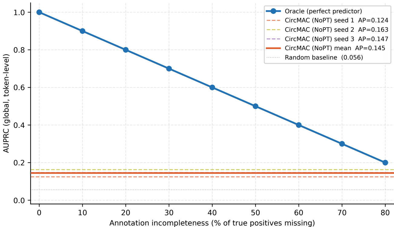
Oracle AUPRC Upper Bound Under Simulated Annotation Noise CircRNA-miRNA Site Prediction (Pair Split, N=7,838 pairs)
