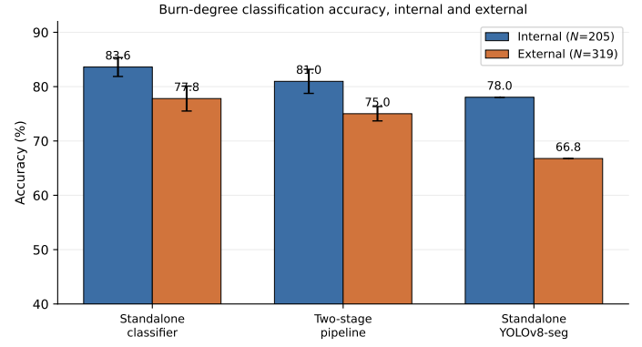
Figure 3: Head-to-head accuracy of the standalone classifier, the robust two-stage pipeline, and the all-in-one YOLOv8-seg model on the internal test set ( N = 205 ) and the clean external set ( N = 319 ). Error bars show the standard deviation across three seeds for the classifier and the pipeline; the standalone YOLOv8-seg model is single-seed and is shown without error bars. The classifier is highest on both sets and leads in every seed. Because the comparison is paired, the correct test is on the per-seed differences rather than on the overlap of these bars: that paired difference is +3.74 percentage points internally (95 percent CI +3.04 to +4.44 ) and +3.24 points externally (95 percent CI -3.83 to +10.31 ).
