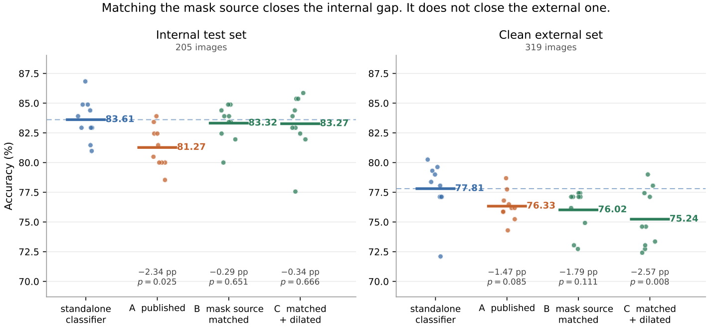
Figure 4: The pipeline as published, against the pipeline given its best configuration. Each dot is one of ten training runs; the heavy bar is the mean; the dashed line is the standalone classifier’s mean. Regime A is the deployed system: its classifier is trained on ground-truth masks and then, at test time, shown masks predicted by the localiser. Regimes B and C remove that mismatch by training on predicted masks, C additionally keeping a 12-pixel rim of skin around the lesion. Internally the repair is worth most of the gap and the difference from the classifier stops being resolvable. Externally it buys nothing: the classifier remains ahead of every regime, and none of the differences between regimes is resolved at ten seeds. Differences beneath each column are paired by seed against the classifier. Note that B is the best regime on test ; validation ranks C first, and against C the external difference from the classifier is resolved (Section 4.5). This is Table 5 drawn.
