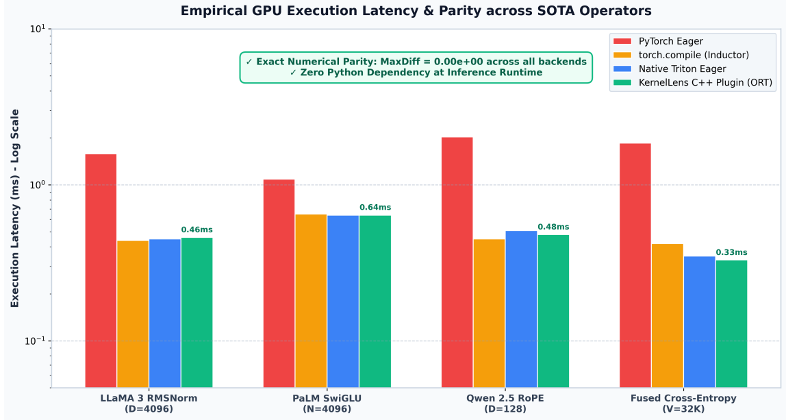
Figure 4: Empirical execution latency comparison (ms, log scale) across PyTorch Eager, torch.compile, Native Triton and KernelLens ONNX Runtime C++ plugins. KernelLens delivers native Triton speed inside C++ runtimes without Python dependencies.
