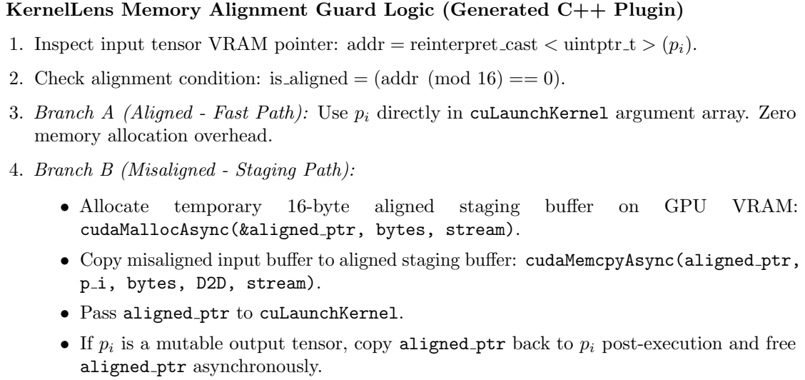
Figure 3: Automated 16-byte memory alignment guard workflow executed in generated C++ plugins.
