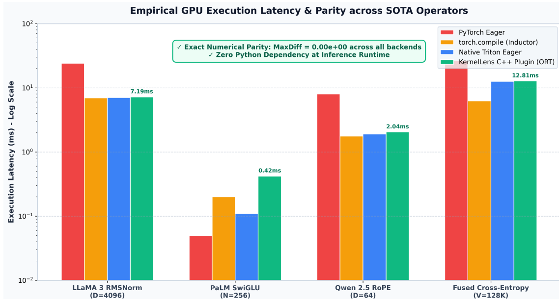
Figure 4: Empirical execution latency comparison (ms, log scale) across PyTorch Eager, torch.compile, Native Triton, and KernelLens ONNX Runtime C++ plugins. KernelLens delivers native Triton speed inside standalone C++ runtimes without Python dependencies.
