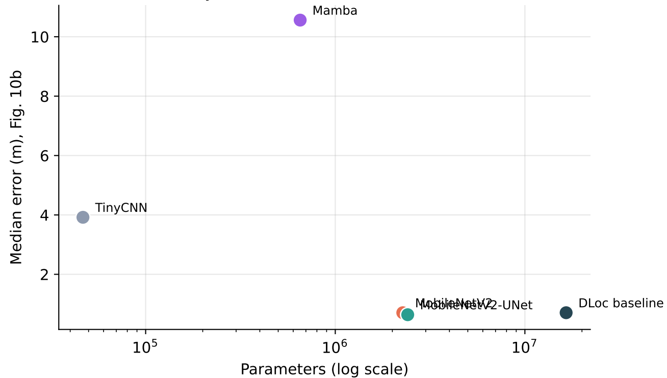
Accuracy vs. model size (lower-left = better)
