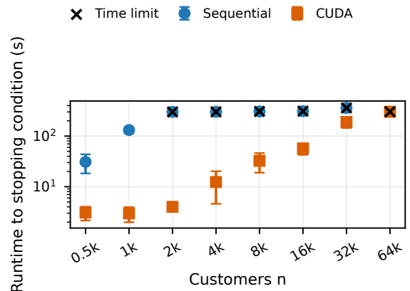
Figure 3: Runtime in the descriptive size sweep. Points are three-run means with sample-SD bars; crosses mark time-limited groups.
