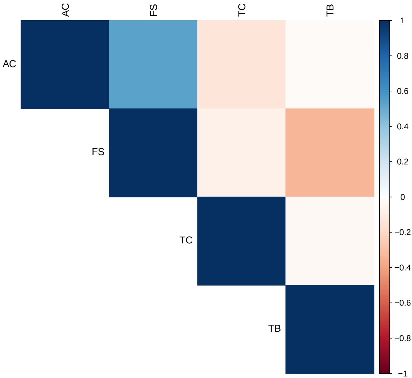
Trait correlations – Baseline
