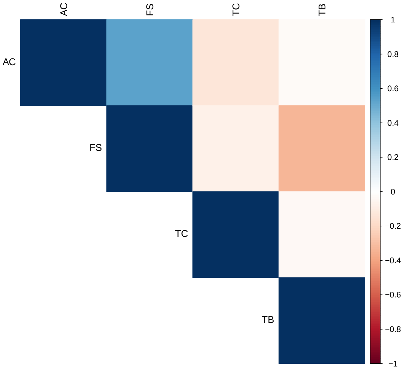
Trait correlations – Long-Term
