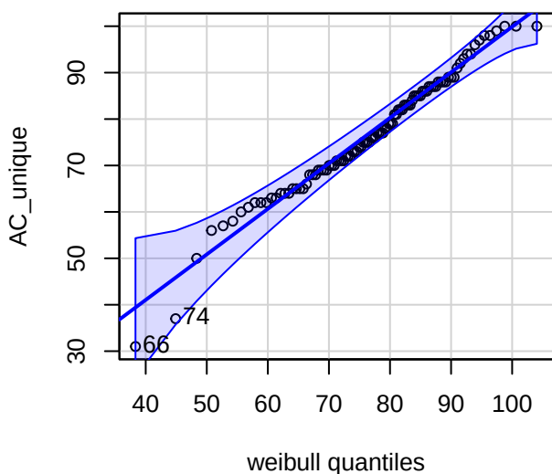
Weibull Q-Q Plot of AC
