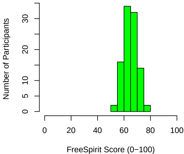
FreeSpirit Score
