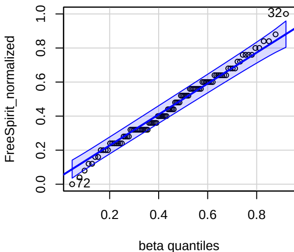
Beta Q-Q Plot of FS
