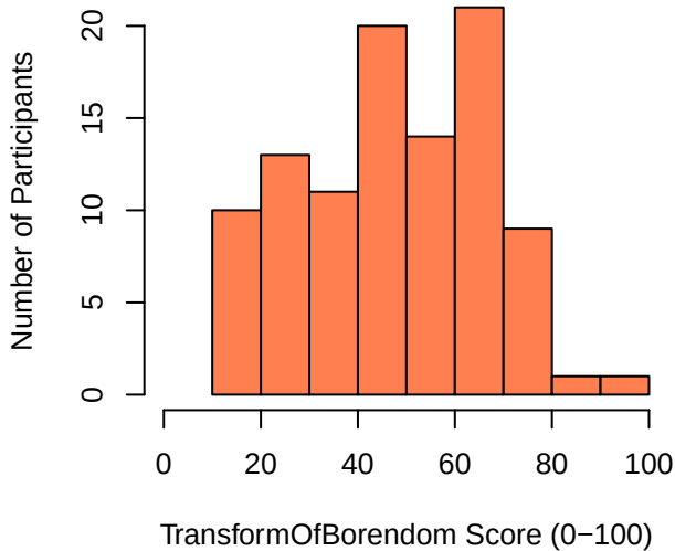
TransformOfBorendom Score
