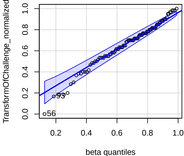
Beta Q-Q Plot of TC
