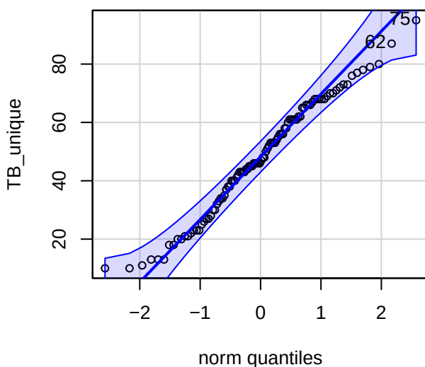
Normal Q-Q Plot of TB
