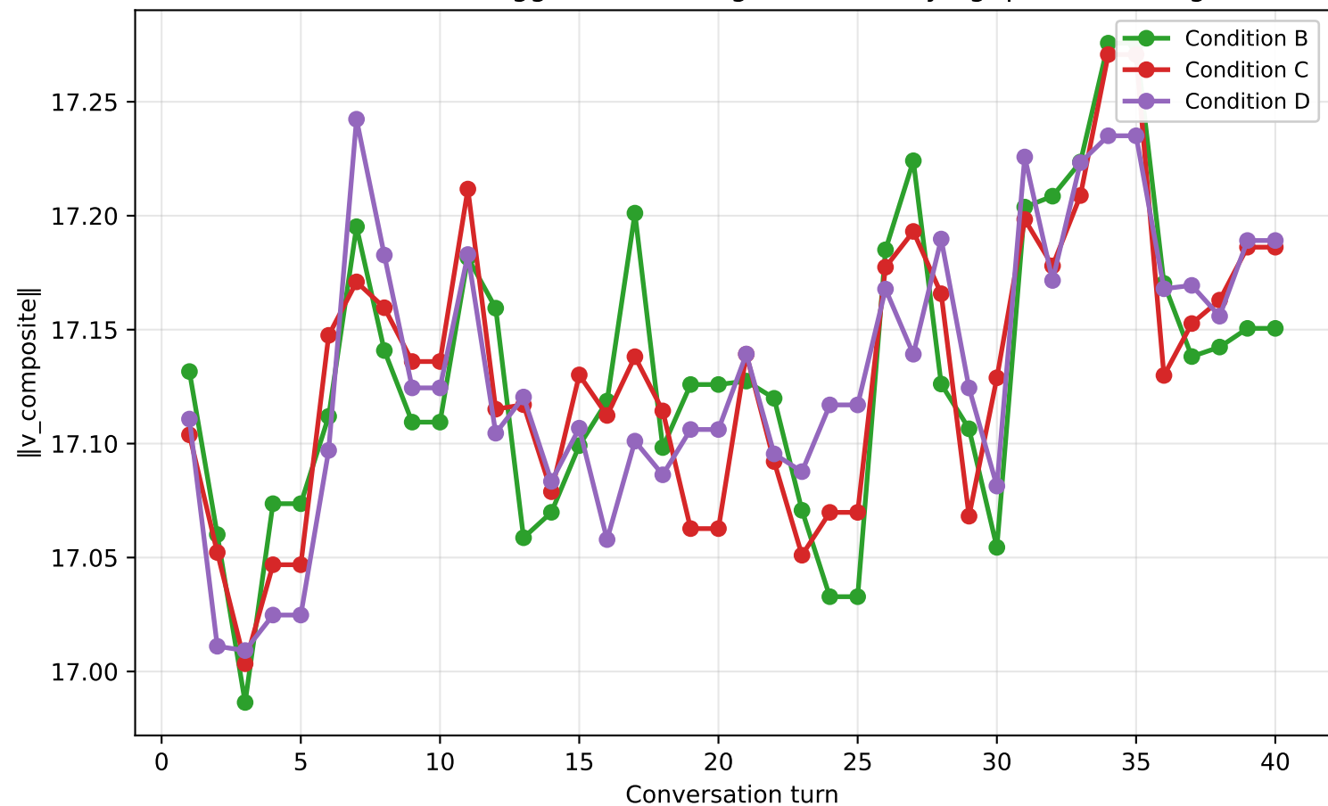
Experiment 5 — composite steering vector norm by turn × condition (near-constant norms suggest QPM marginals not varying; plan §8.5 diagnostic)
