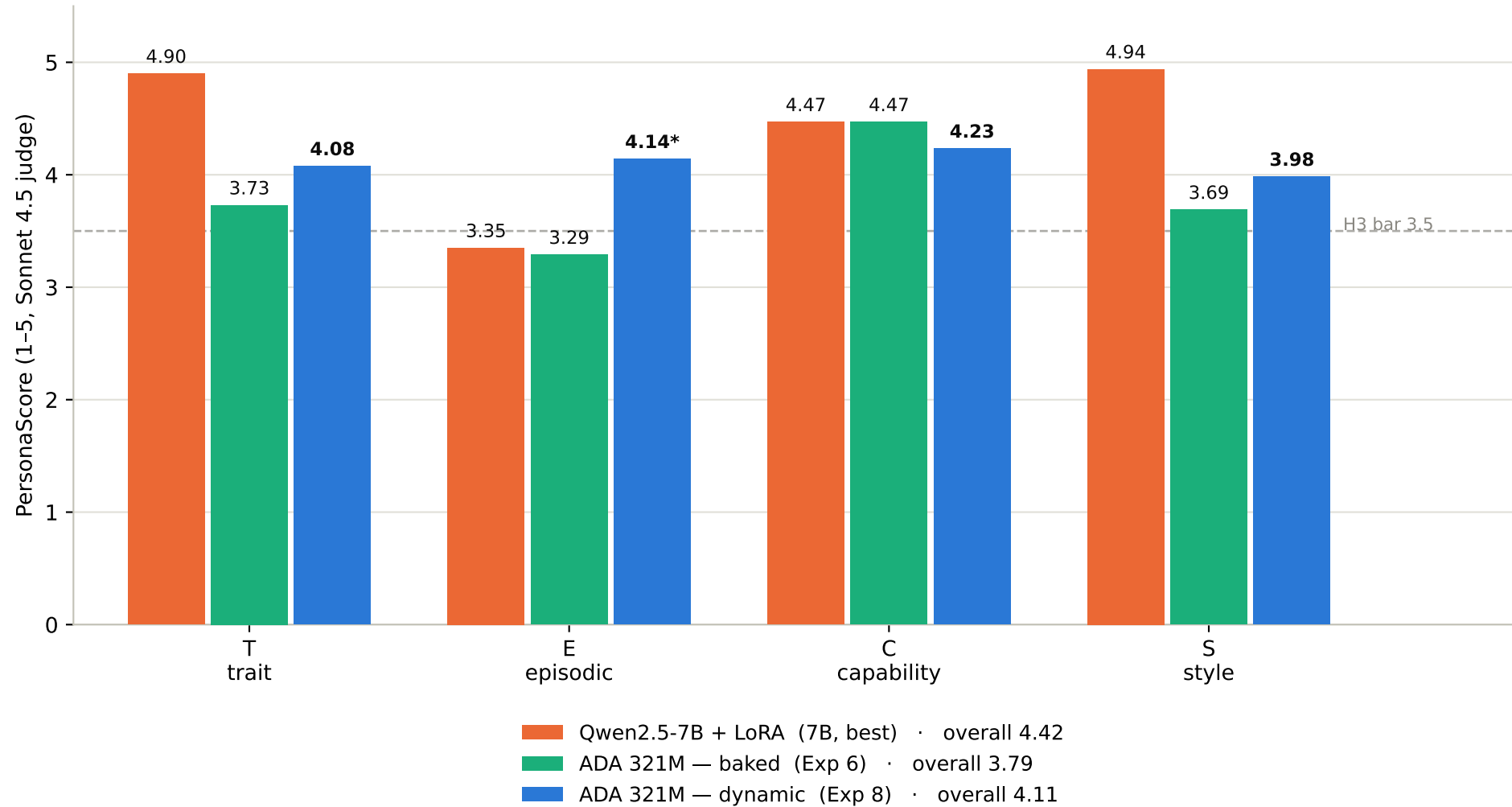
PersonaScore by dimension — Qwen2.5-7B vs owned ADA 321M (baked → dynamic)
