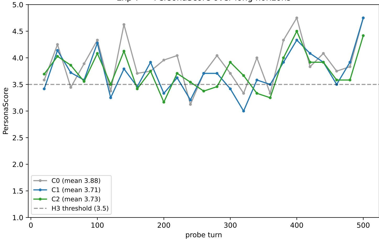
Exp 7 — PersonaScore over long horizons
