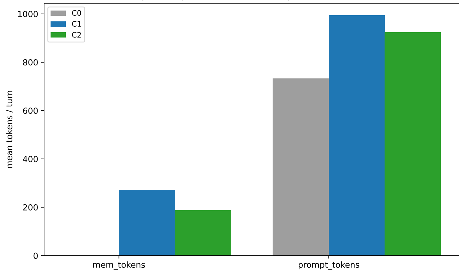
Exp 7 — injected-context cost by condition (RQ4)
