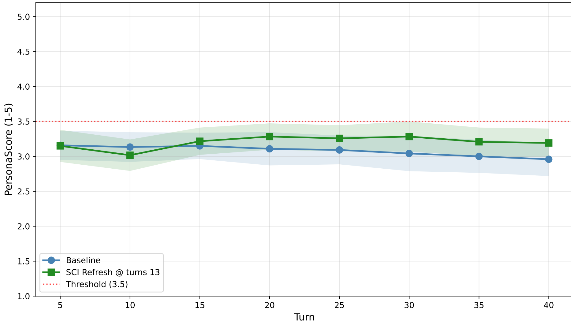
Baseline vs. SCI Refresh @ turns 13
