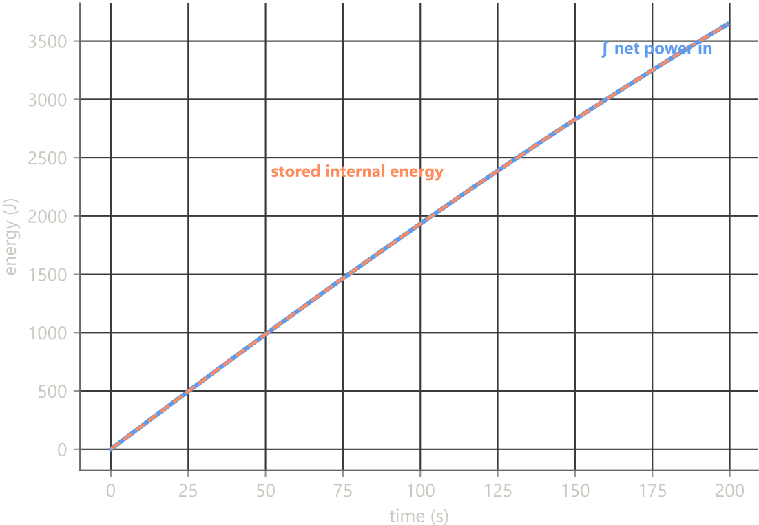
Heater + ambient radiation + conduction, all active
