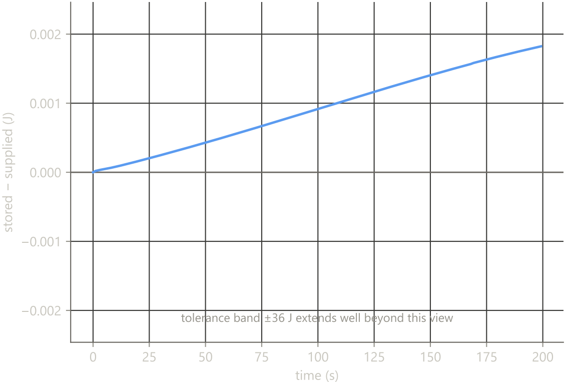
Imbalance peaks at 1.8\text{e-}03 J — 19980× inside the \pm 36 J tolerance
