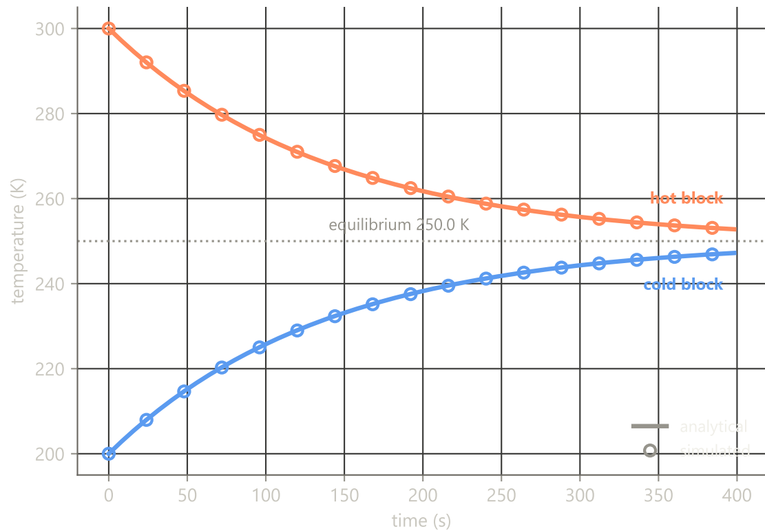
Contact-coupled pair relaxing to equilibrium (max |error| = 0.057 K)
