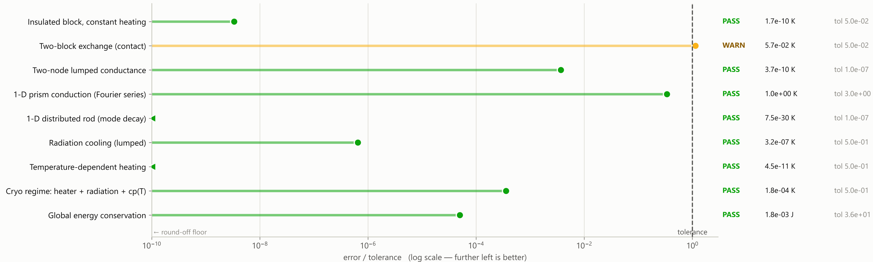
Thermal solver vs. closed-form references: 8/9 within tolerance, 1 marginal
