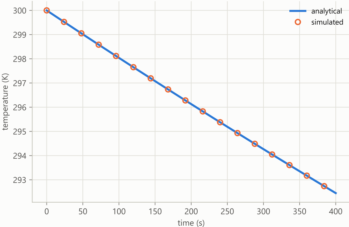
Radiation cooling (lumped) max |error| = 3.2e-07 K
