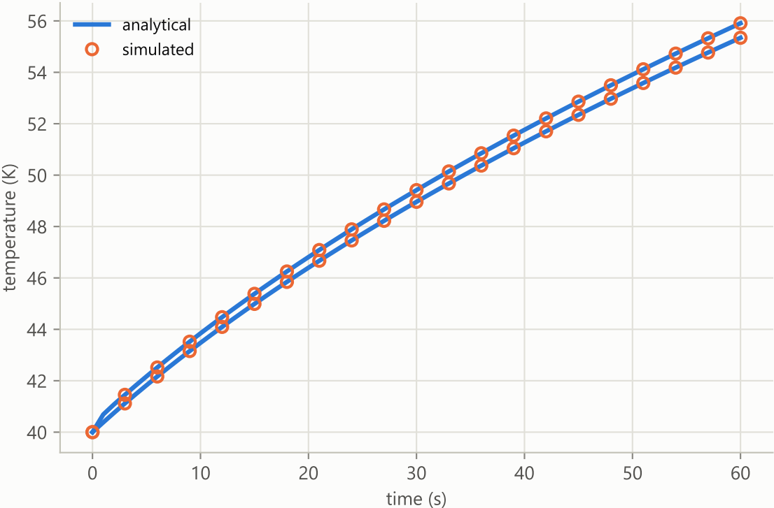
Cryo regime: heater + radiation + cp(T) max |error| = 2.9e-04 K
