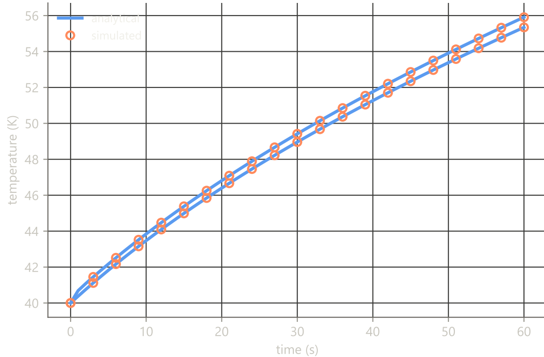
Cryo regime: heater + radiation + cp(T) max |error| = 2.9 \times 10^{-4} K
