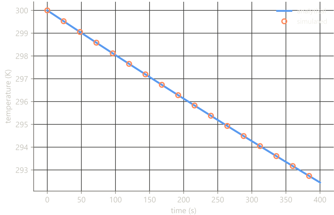
Radiation cooling (lumped) max |error| = 3.2 \times 10^{-7} K
