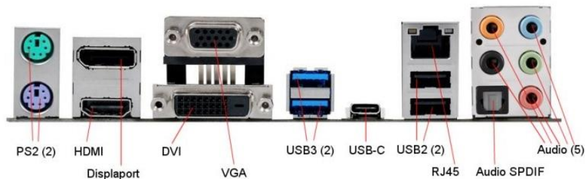
Ports externes
